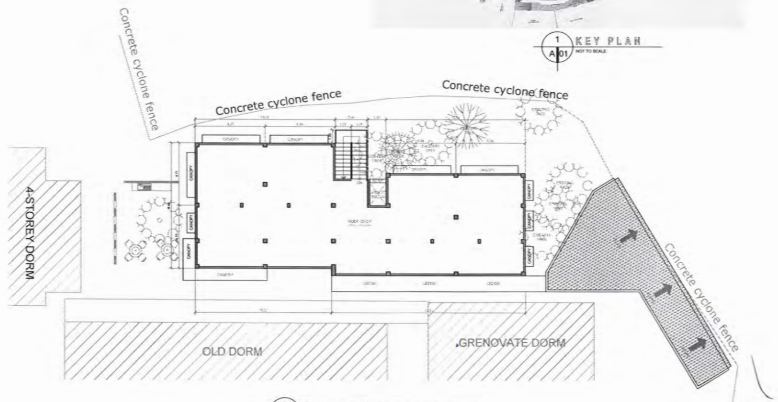
2 SITE DEVELOPMENT PLAN A 01 SCALE 1:100 METERS
