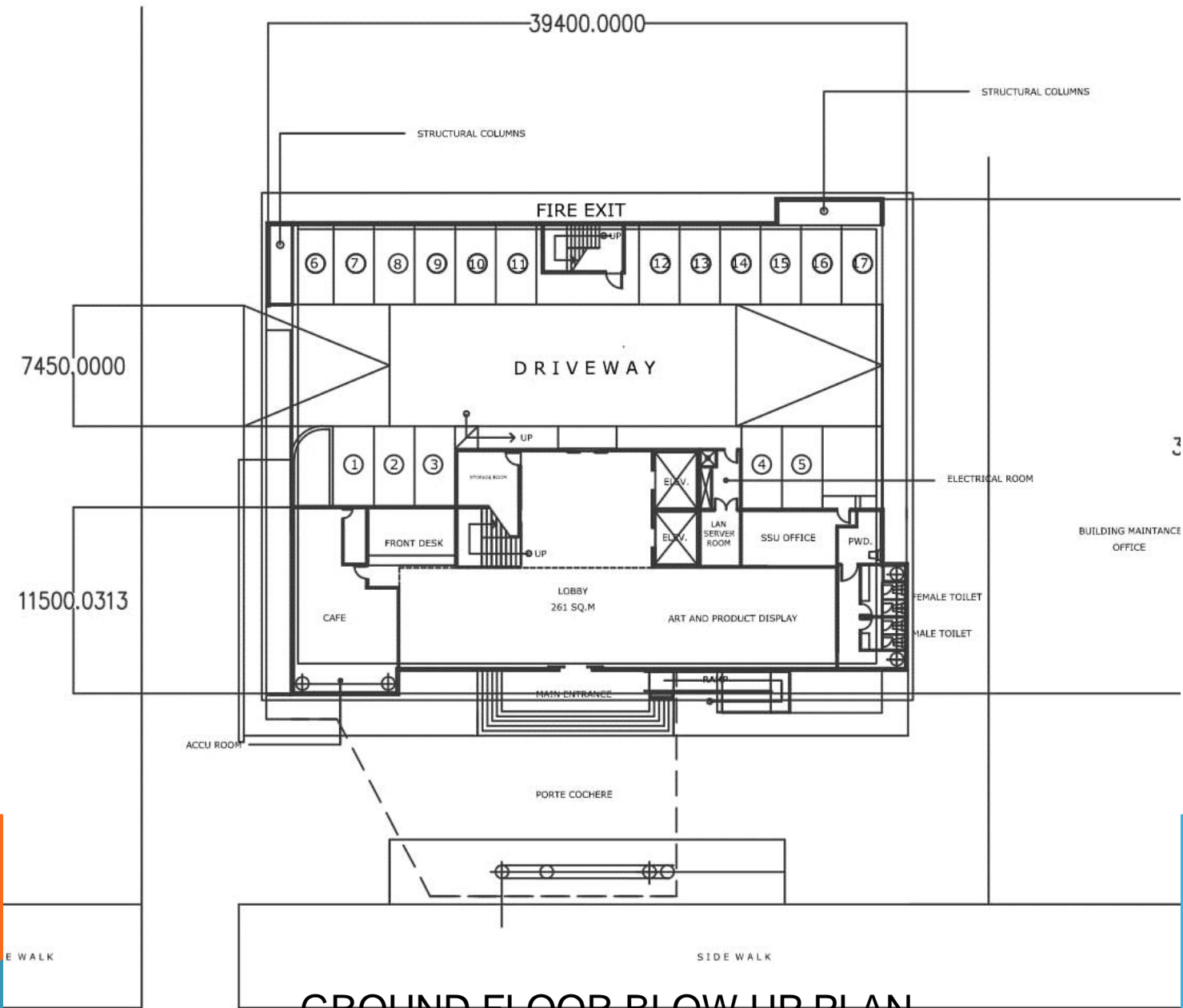
GROUND FLOOR BLOW-UP PLAN
